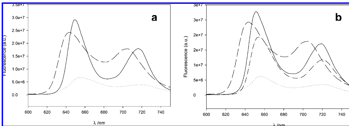
Figure 3. Fluorescence emission spectra of 1 \mu\text{M H}_2\text{TPPS}_4^{4-} in water (panels a and b, dashed line) and in the presence of (a) surfactant 1a at [surfactant]/[porphyrin] ratio of 4:1, \lambda_{\text{ex}} 408 nm (dotted line), at surfactant/porphyrin ratio of 10 000:1, \lambda_{\text{ex}} = 413 nm (solid line); (b) surfactant 2 at [surfactant]/[porphyrin] ratio of 4:1, \lambda_{\text{ex}} 408 nm (dotted line), at [surfactant]/[porphyrin] ratio of 10 000:1, \lambda_{\text{ex}} 407 nm (dash-dotted line), and \lambda_{\text{ex}} = 420 nm (solid line).
